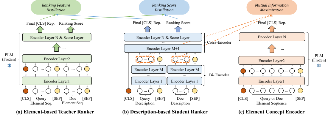
Figure 4: The training framework of Elem4LCR-I. We propose an element knowledge enhancement method based on mutual information maximization, a multi-level element interaction legal distillation method, and a customized training curriculum to comprehensively improve the model training with legal elements.
